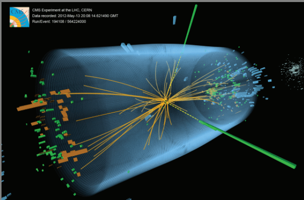
Higgs boson detection (CERN)
